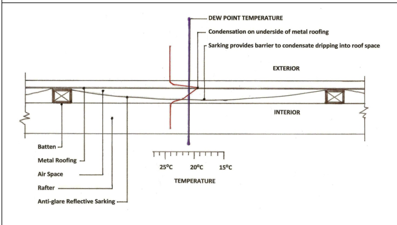
Figure A.16 Sarking under metal roof
