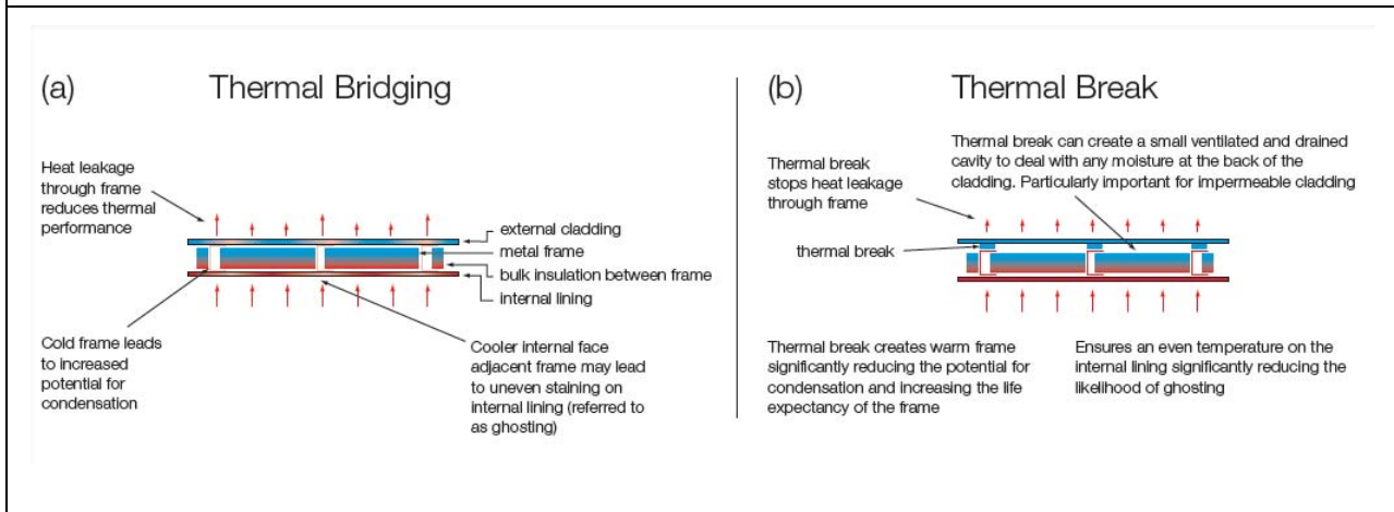
Figure 5.2 Thermal breaks improve clad wall performance.
